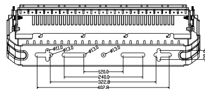
Fixture fixed hole size diagram
