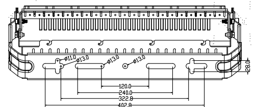
Fixture fixed hole size diagram
